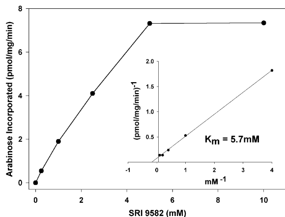
Figure 4. Kinetic analysis of acceptor SRI-9582 . The inset illustrates the double reciprocal plot for SRI-9582 as a substrate for the mycobacterial arabinosyltransferase.
